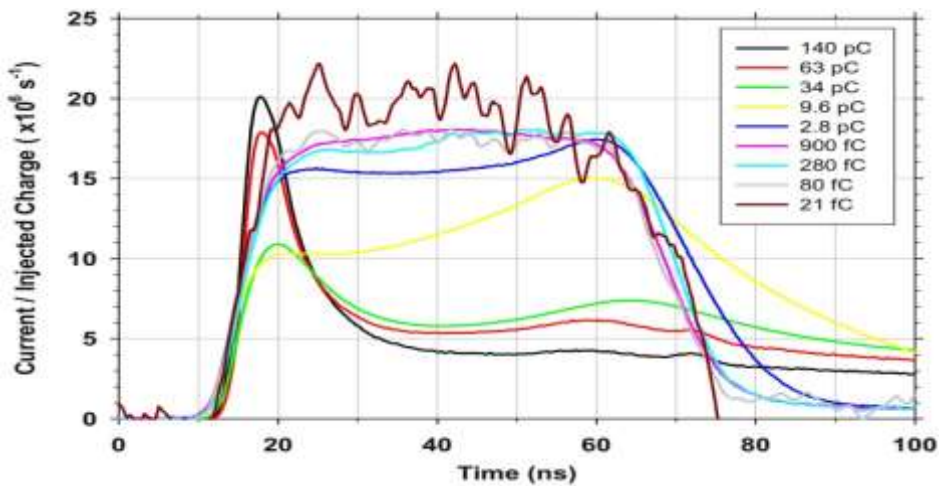
Figure1: Transient-current signal (holes) at 34 V for varying laser intensities, illustrating the transition from SCFC to SCLC currents at Q_{inj} = 34\text{pC} , figure adapted from [Isberg et al., 2011].
